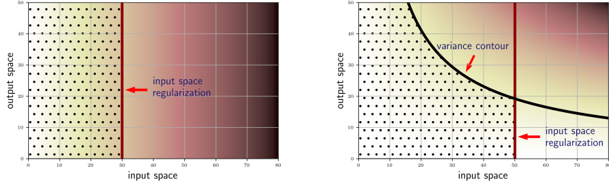
Figure 1: An illustration of our proposed regularization scheme. Left: the regularized least-squares estimator studied in previous works (Fischer & Steinwart, 2020; de Hoop et al., 2021; Talwai et al., 2022) which only regularizes on the input space. Right: our double regularization scheme via variance contour can achieve the optimal convergence rate in our setting.
