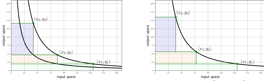
Figure 3: Construction of the sequence \{(x_i, y_i)\} . Left: the case \frac{\beta-\beta'}{\max\{\alpha, \beta+p\}} \neq \frac{\gamma'-\gamma}{1-\gamma} . Right: the case \frac{\beta-\beta'}{\max\{\alpha, \beta+p\}} = \frac{\gamma'-\gamma}{1-\gamma} , where the bias and variance contours overlap and we set x_{n+1} = \frac{1}{2}x_n . Each rectangular represents a certain level of regularization.
